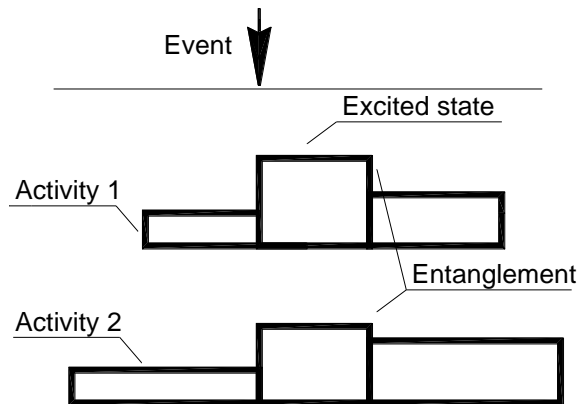
Figure 11. Entanglement effect
